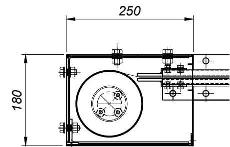
1 Headbox Roller Assembly End Detail
