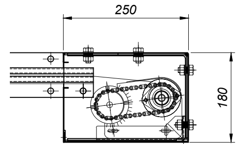
2 Headbox Pulley Assembly End Detail
