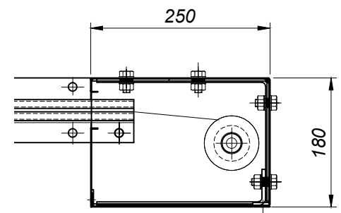
Section D Pulley System
